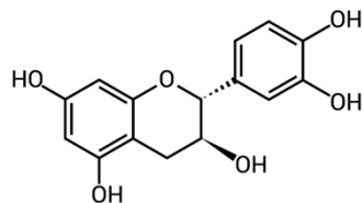
Catechin
